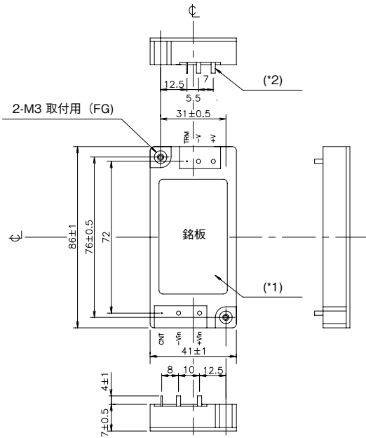
[PH75S] (Package Type:T41)
