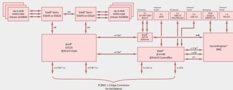
PCIe® 2.0 Backplane
