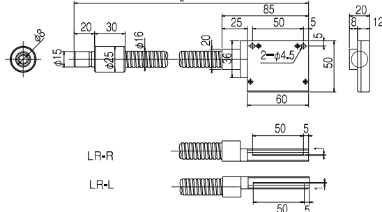
LGB1-8L1000-LR-R80×0.6 LGC1-8L1000-LR-R80×0.6 LGB1-8L1000-LR-L80×0.6 LGC1-8L1000-LR-L80×0.6
