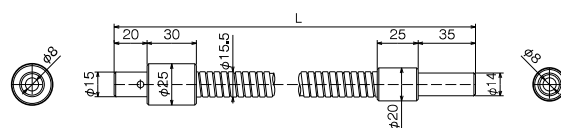
LGA1-8L500N
