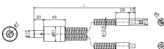
LGA2-5L500N/1000N PLGA2-5L500N
