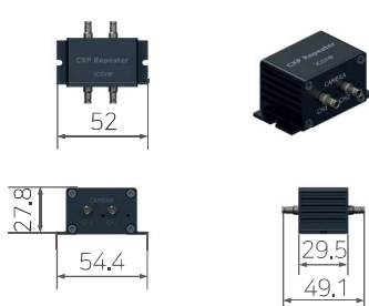
Figure 2 iPLUS-CXPR-DIN2
