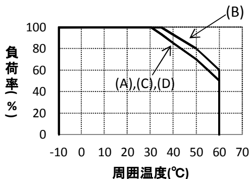
LFS150A-12
