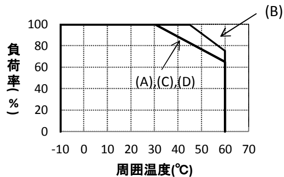
LFS150A-24
