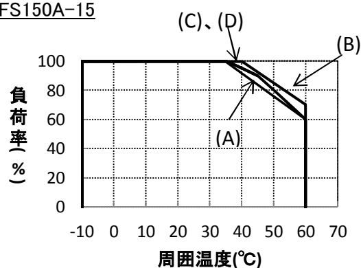
LFS150A-15
