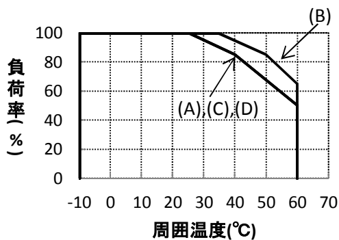
LFS150A-5
